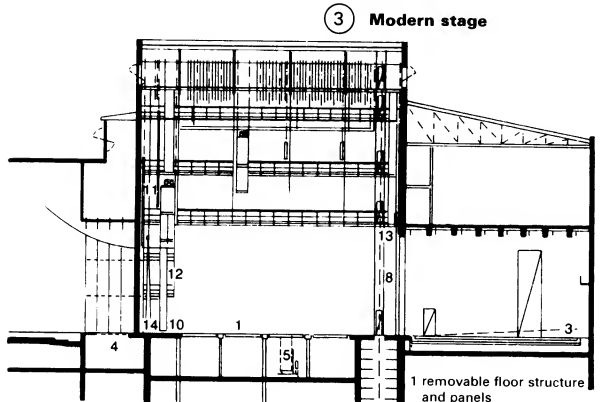
④ Typical three-section theatre (section) → ⑤
